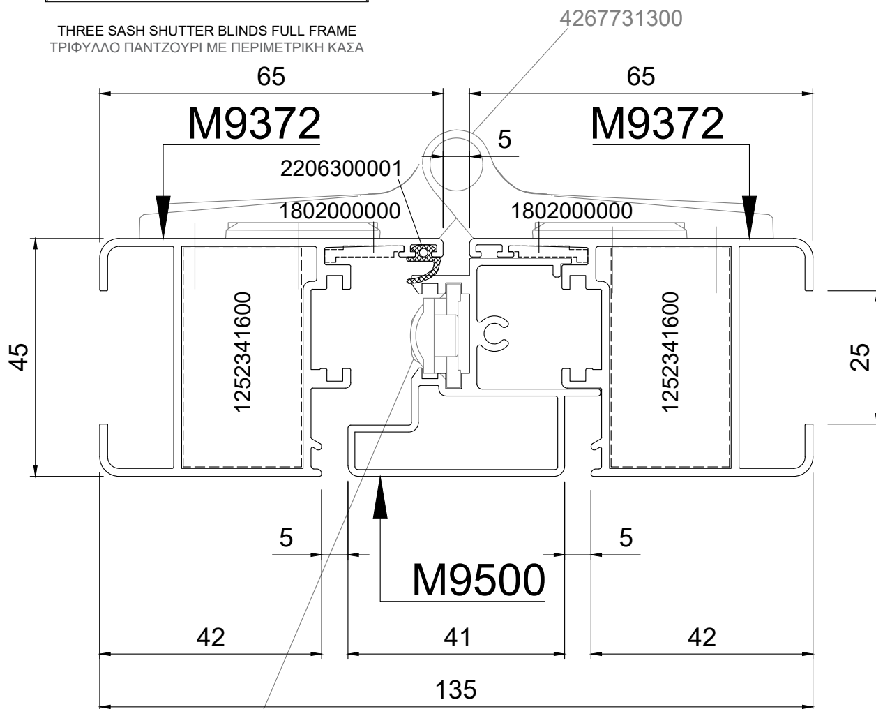
Folding Position
