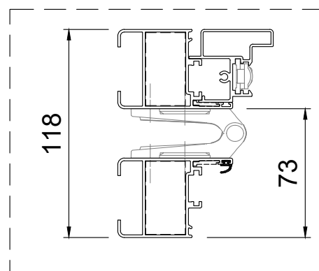
Folding Position
