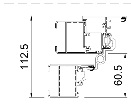
Folding Position
