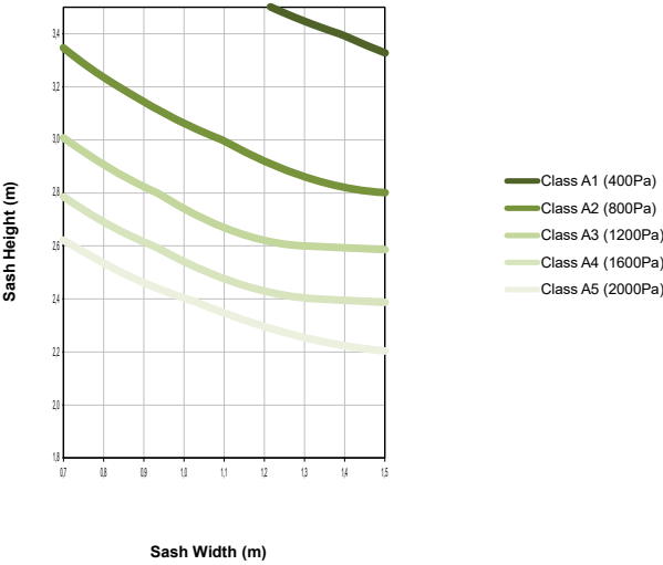
Maximum Panel Dimensions For Given Wind Pressure Class A ... L/150 deflection limit
