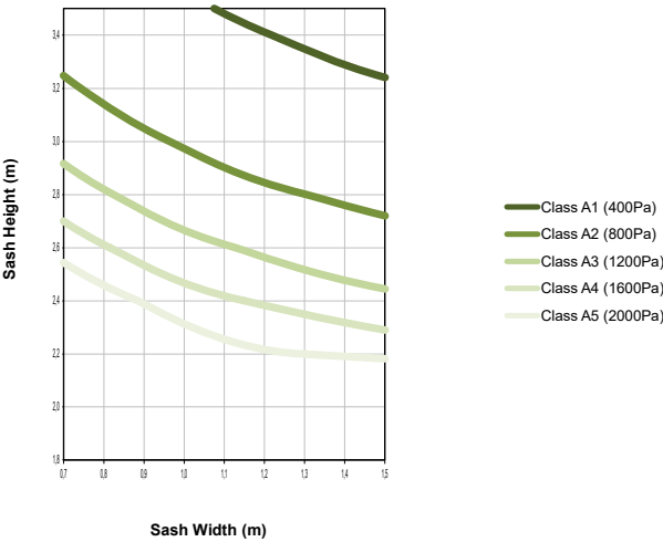
Maximum Panel Dimensions For Given Wind Pressure Class A ... L/150 deflection limit
