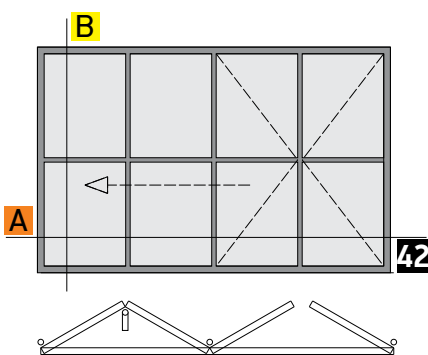
OUTWARD OPENING, 3+1 4-PANELS FOLDING DOOR ΕΞΩ ΑΝΟΙΓΟΜΕΝΗ, 3+1 4-ΦΥΛΛΗ ΦΥΣΟΥΝΑ
