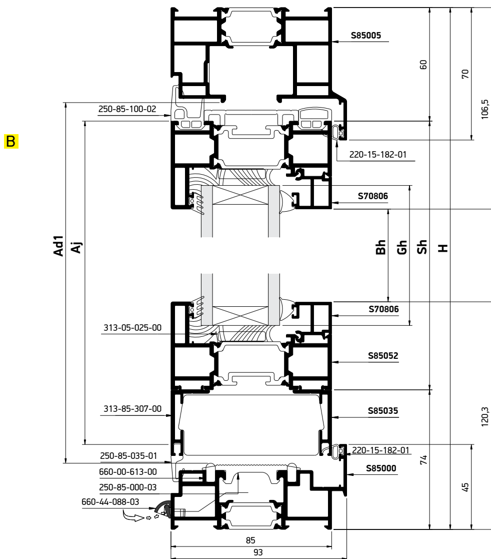
OUTWARD OPENING, 3+1 4-PANELS FOLDING DOOR ΕΞΩ ΑΝΟΙΓΟΜΕΝΗ, 3+1 4-ΦΥΛΛΗ ΦΥΣΟΥΝΑ
