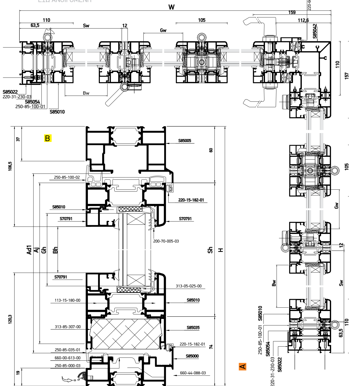
3+3 CORNER TYPOLOGY OUTWARD OPENING
