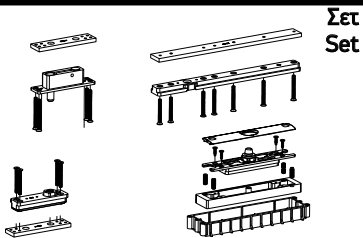
Pivot mechanism set
