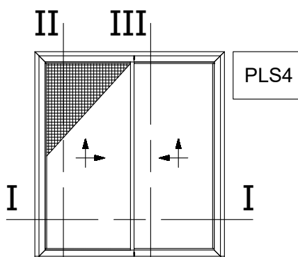
Two Sash Parallel Lift and Slide 90 Degrees Cut Right Sliding Window with Flyscreen
