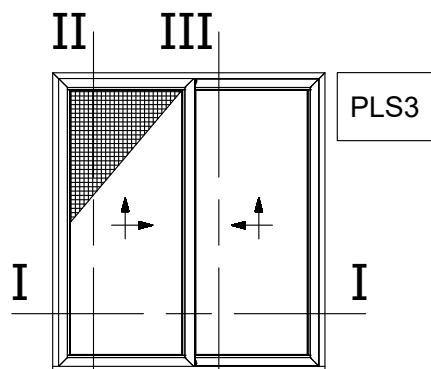
Two Sash Parallel Lift and Slide 45 Degrees Cut Right Sliding Window with Flyscreen
