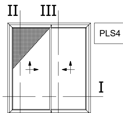
II III Two Sash Parallel Lift and Slide 90 Degrees Cut Right Sliding Window with Flyscreen
