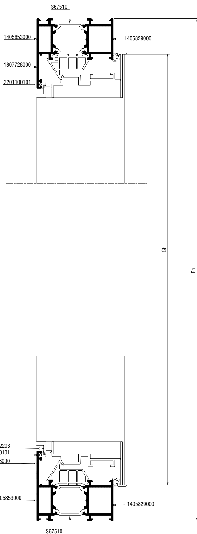
Window wall with ventilation flap
