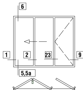
OUTWARD OPENING 2 +1 3-PANELS FOLDING DOOR ΕΞΩ ΑΝΟΙΓΟΜΕΝΗ 2+1 3-ΦΥΛΛΗ ΦΥΣΟΥΝΑ
