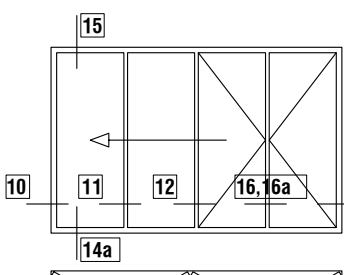
INWARD OPENING 3+1 4-PANELS FOLDING DOOR ΕΞΩ ΑΝΟΙΓΟΜΕΝΗ 3+1 4-ΦΥΛΛΗ ΦΥΣΟΥΝΑ
