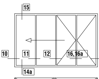
INWARD OPENING 3+1 4-PANELS FOLDING DOOR ΕΞΩ ΑΝΟΙΓΟΜΕΝΗ 3+1 4-ΦΥΛΛΗ ΦΥΣΟΥΝΑ
