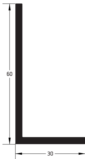
Γ-60x30x3
