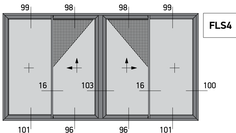
Four Sash Meeting Stile Monorail Lift and Slide with Flyscreen
