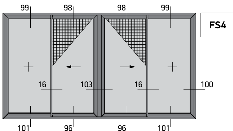
Four Sash Sliding Meeting Stile Monorail with Flyscreen
