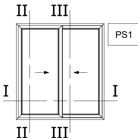
Two Sash Sliding Window 45° Cut Right
