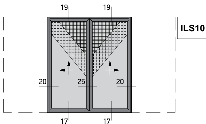
Pocket Lift&Slide Window with Meeting Stile, with Narrow Flyscreen and Shutter
