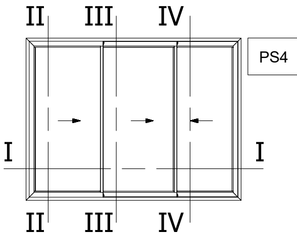
Three Sash Sliding Window 90° Cut Right
