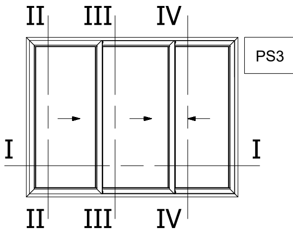
Three Sash Sliding Window 45° Cut Right
