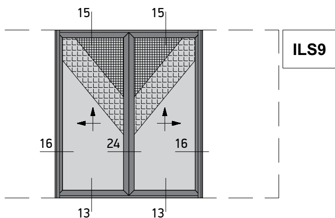
Pocket Lift&Slide Window with Meeting Stile, with Flyscreen and Shutter
