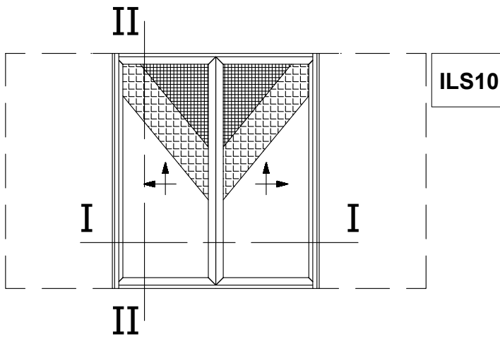
Pocket Lift&Slide Window with Meeting Stile, with Narrow Flyscreen and Shutter
