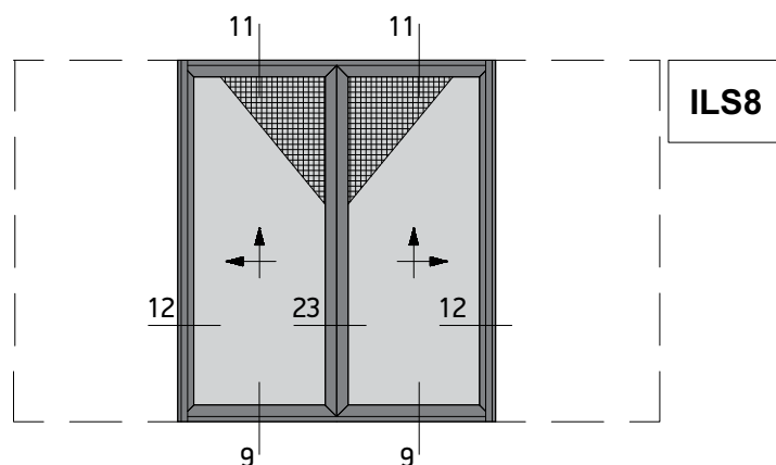
Pocket Lift&Slide Window with Meeting Stile and Narrow Flyscreen
