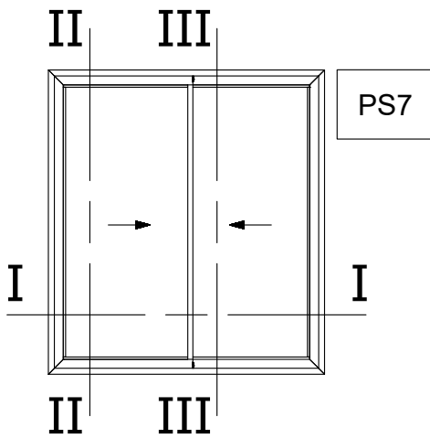
Two Sash Sliding Window 90° Cut (Sash M4544) Right
