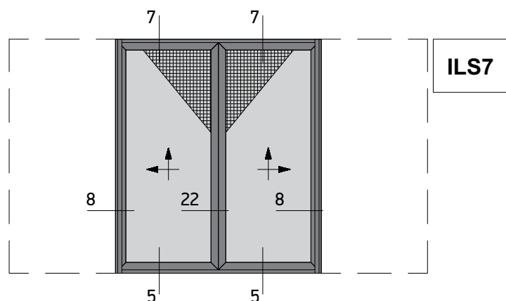
Pocket Lift&Slide Window with Meeting Stile and Flyscreen
