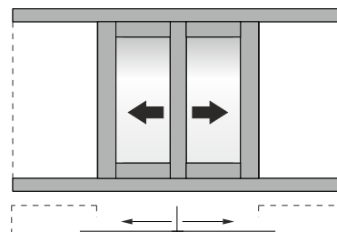
Double narrow sash pocket sliding in 90° assembly window in meeting stile Δίφυλλο χωνευτό με 90° κοπή
