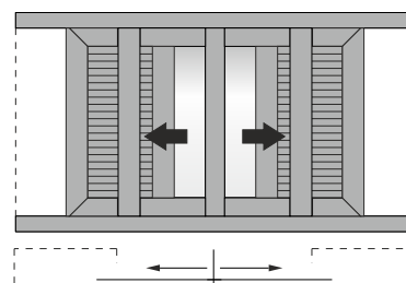
Double narrow sash pocket sliding in 90° assembly window in meeting stile with shutters Δίφυλλο χωνευτό με 90° κοπή, με παντζούρι
